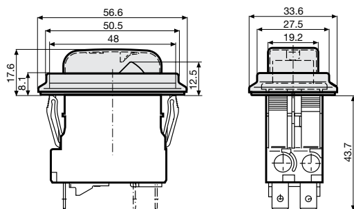
Accessories / factory mounted AZM01 / Collar with cover, IP54
