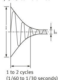
(6) Electromagnetic Contact Load i/i_o \approx 3 to 10 times
