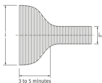
(2) Mercury Lamp Load i/i_o \approx 3 times
