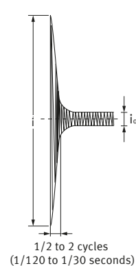
(7) Capacitive Load i/i_o \approx 20 to 40 times
