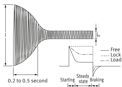
(4) Motor Load i/i_o \approx 5 to 10 times
