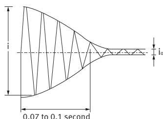
(5) Solenoid Load i/i_o \approx 10 to 20 times
