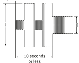
(3) Fluorescent Lamp Load i/i_o \approx 5 to 10 times
