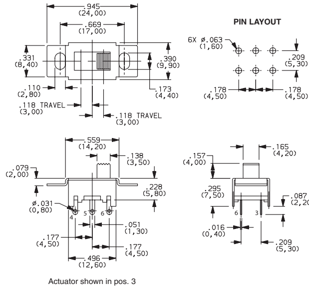
OS203013MT7QN1 DP3T
