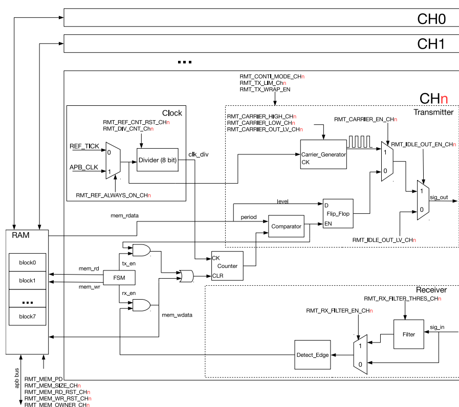
Figure 90: RMT Architecture
