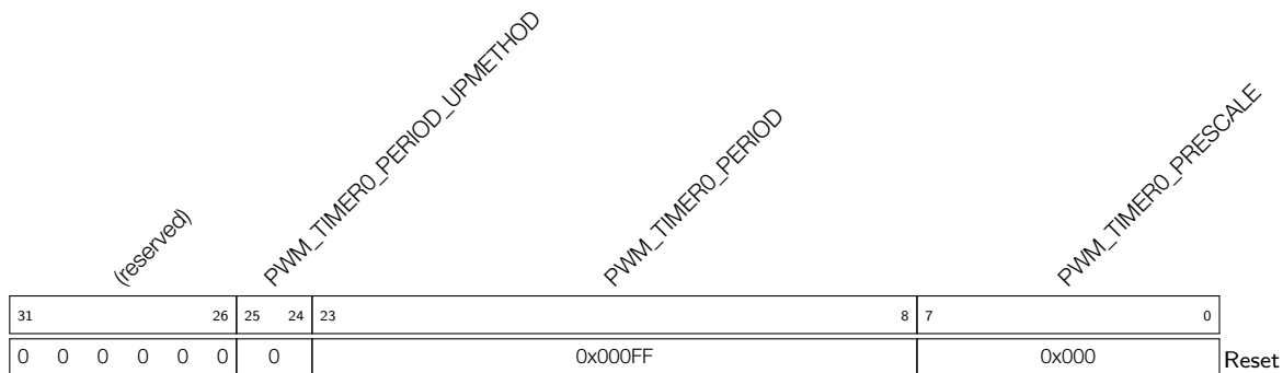
Register 16.2: PWM_TIMER0_CFG0_REG (0x0004)
