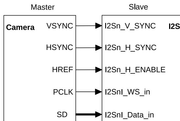
Figure 76: Camera Slave Receiving Mode
