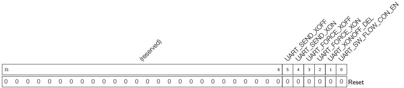
Register 13.14: UART_FLOW_CONF_REG (0x34)
