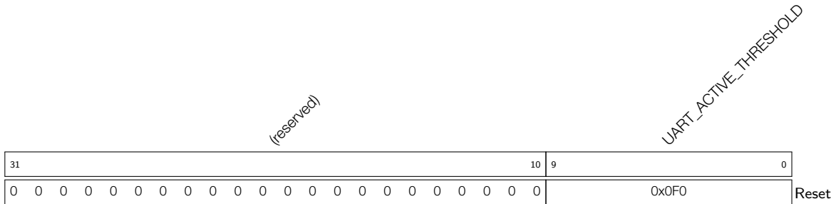
Register 13.15: UART_SLEEP_CONF_REG (0x38)
