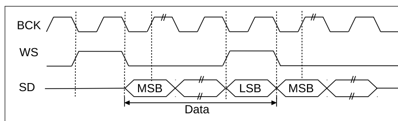
Figure 65: PCM Standard
