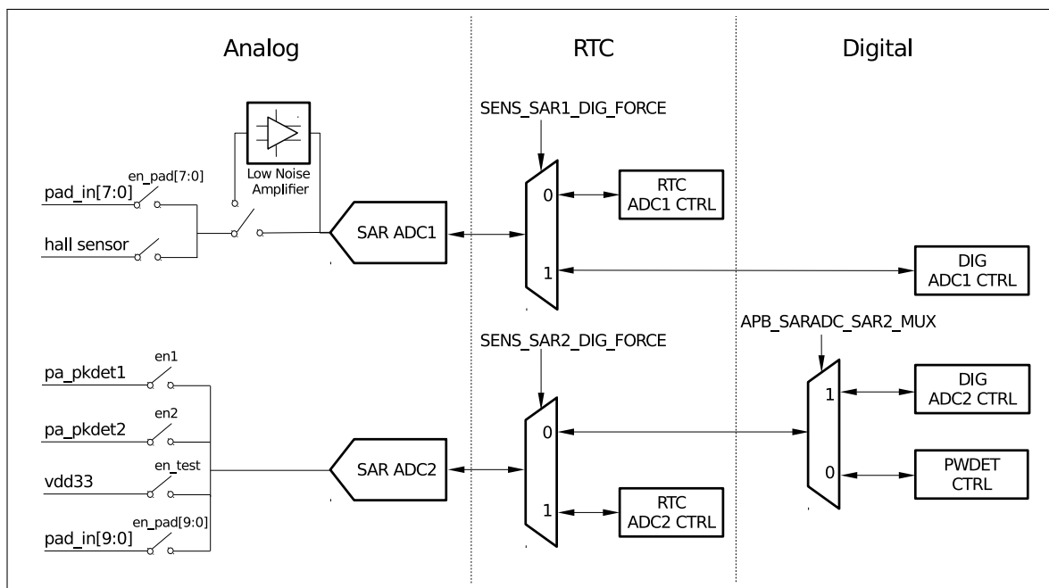
Figure 132: SAR ADC Outline of Function
