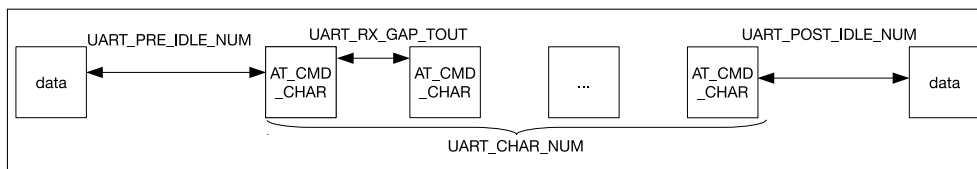
Figure 83: AT_CMD Character Format
