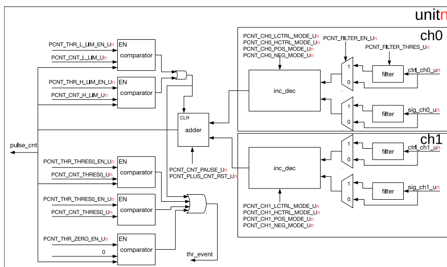
Figure 121: PULSE_CNT Architecture
