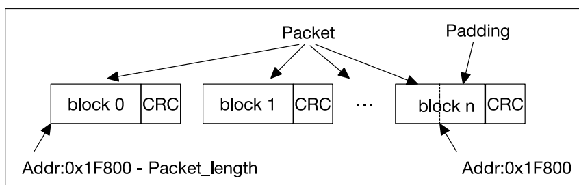
Figure 23: SDIO Bus Packet Transmission
