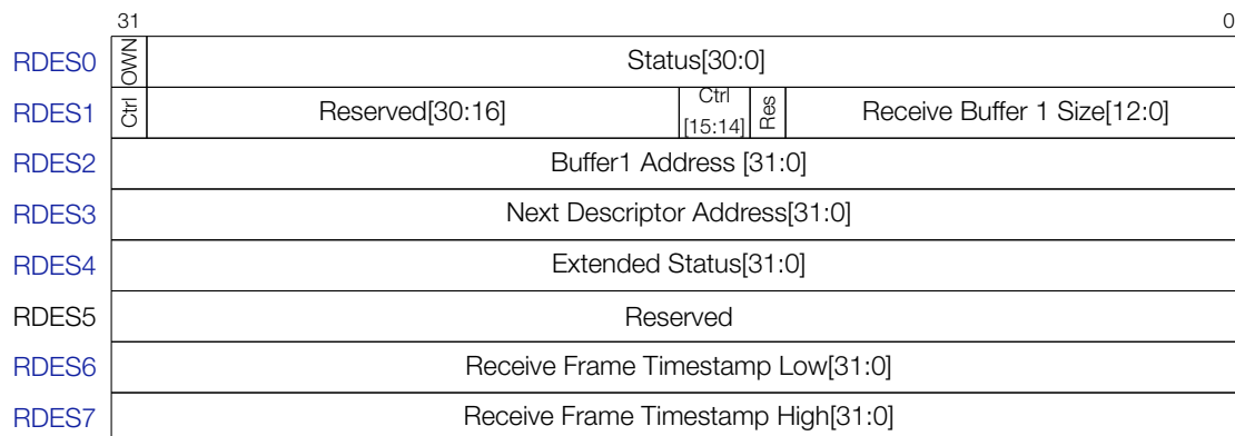
Figure 48: Receive Descriptor
