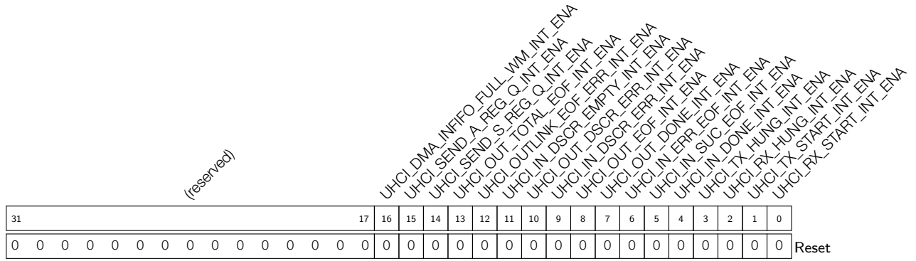
Register 13.30: UHCI_INT_ENA_REG (0xC)
