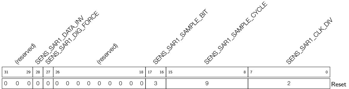
Register 28.1: SENS_SAR_READ_CTRL_REG (0x0000)
