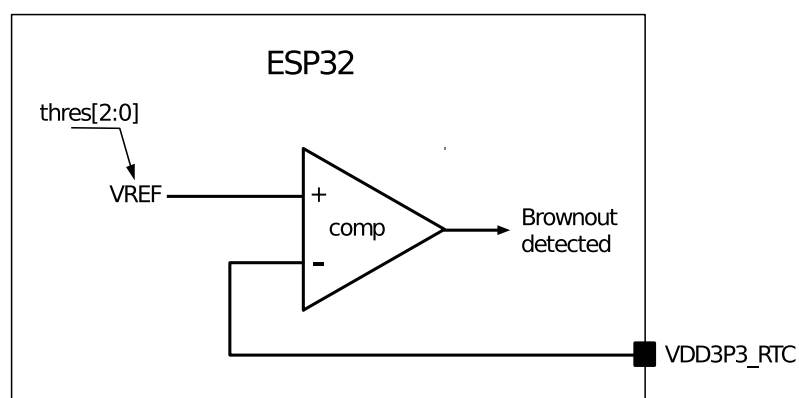
Figure 164: Brownout Detector
