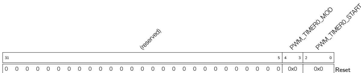
Register 16.3: PWM_TIMER0_CFG1_REG (0x0008)
