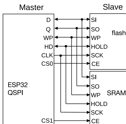
Figure 20: Parallel QSPI
