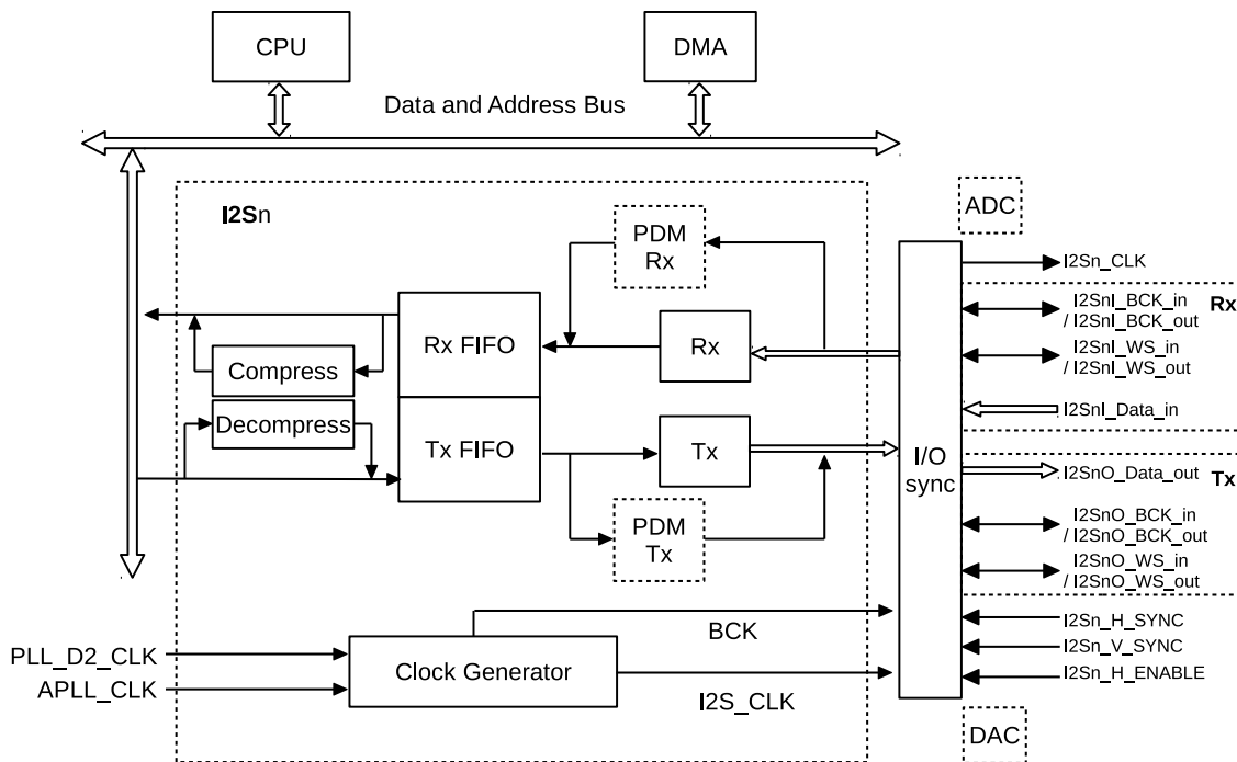
Figure 61: I2S System Block Diagram
