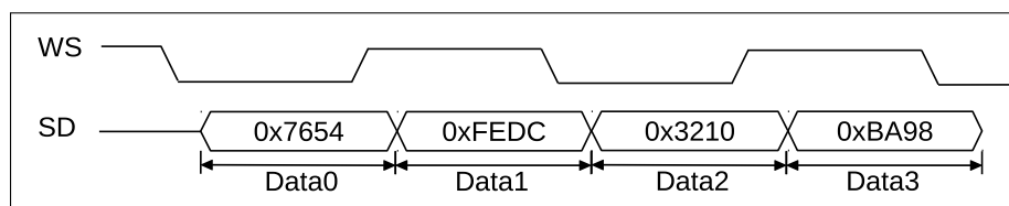
Figure 67: The First Stage of Receiving Data
