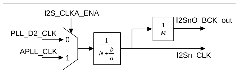
Figure 62: I2S Clock
