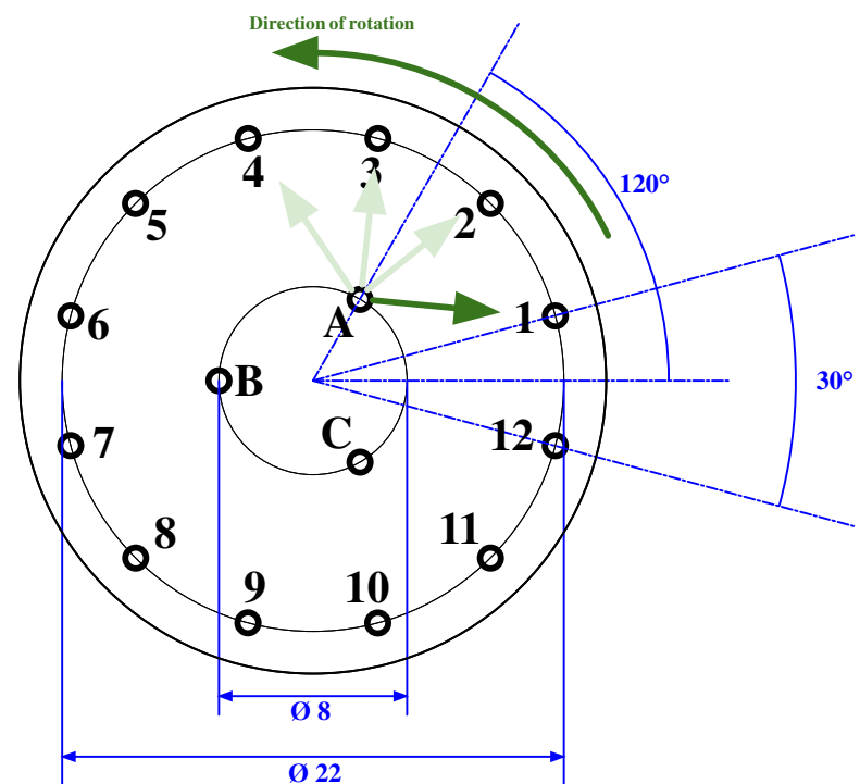
Bottom view
