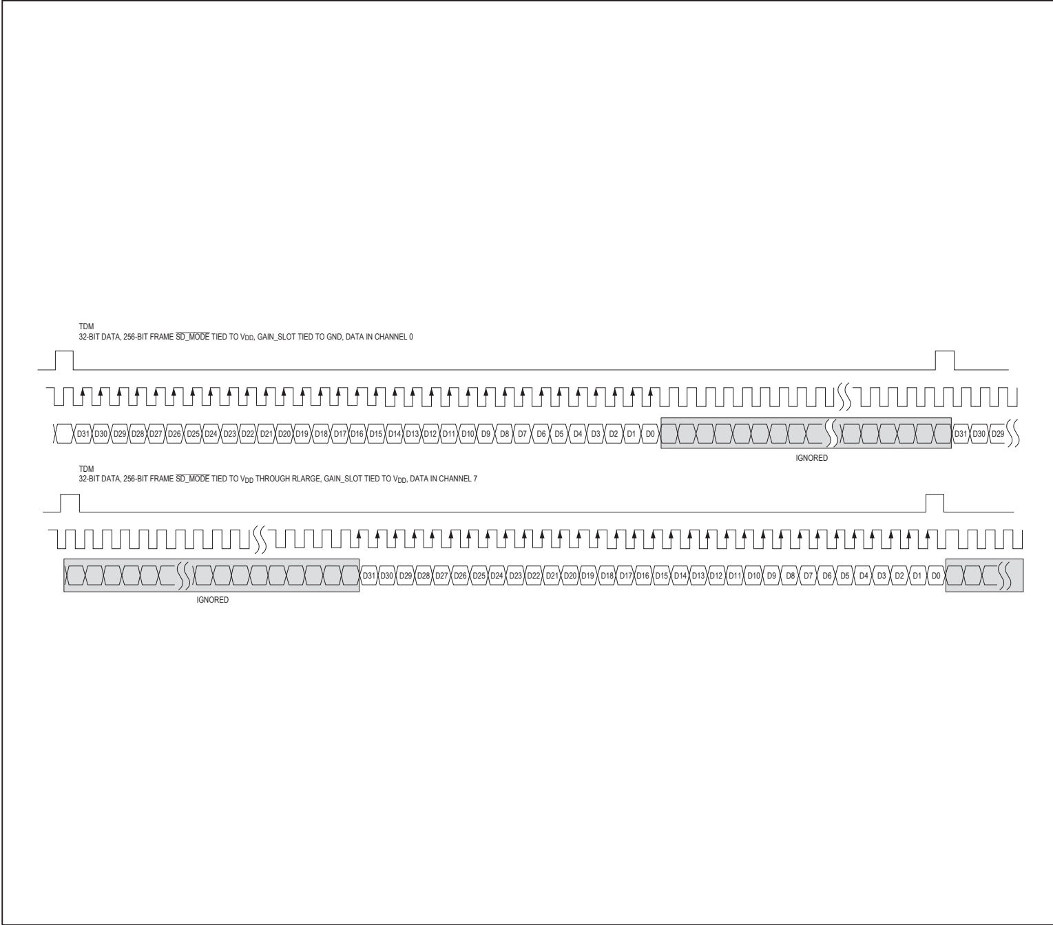
Figure 12. MAX98357A TDM 32-Bit DAI Timing
