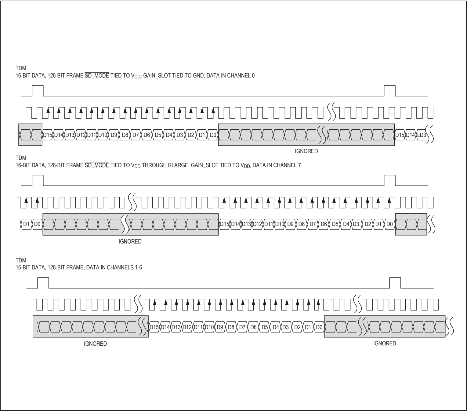
Figure 11. MAX98357A TDM 16-Bit DAI Timing
