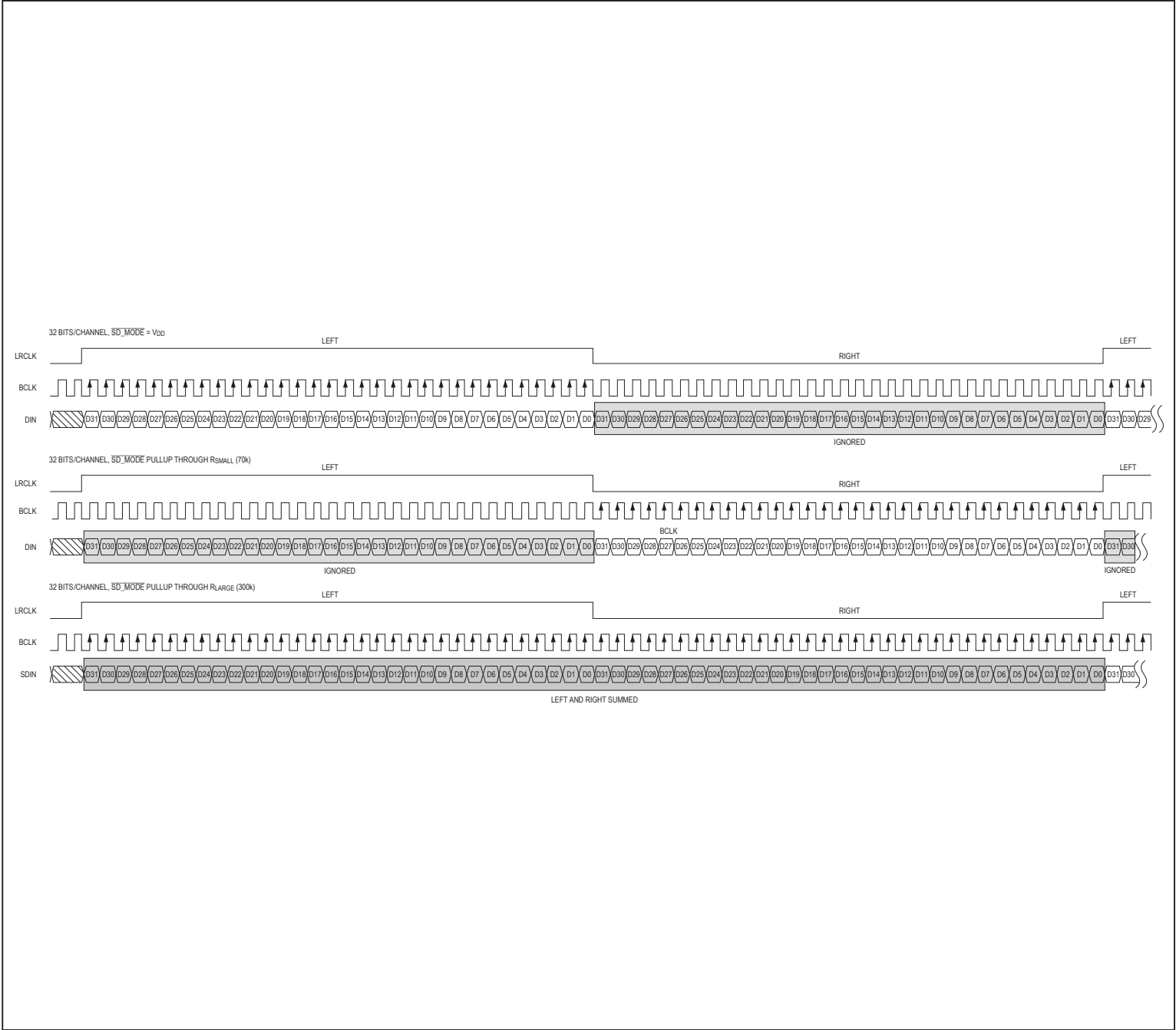
Figure 10. MAX98357B Left-Justified Digital Audio Interface Timing, 32-Bit Resolution
