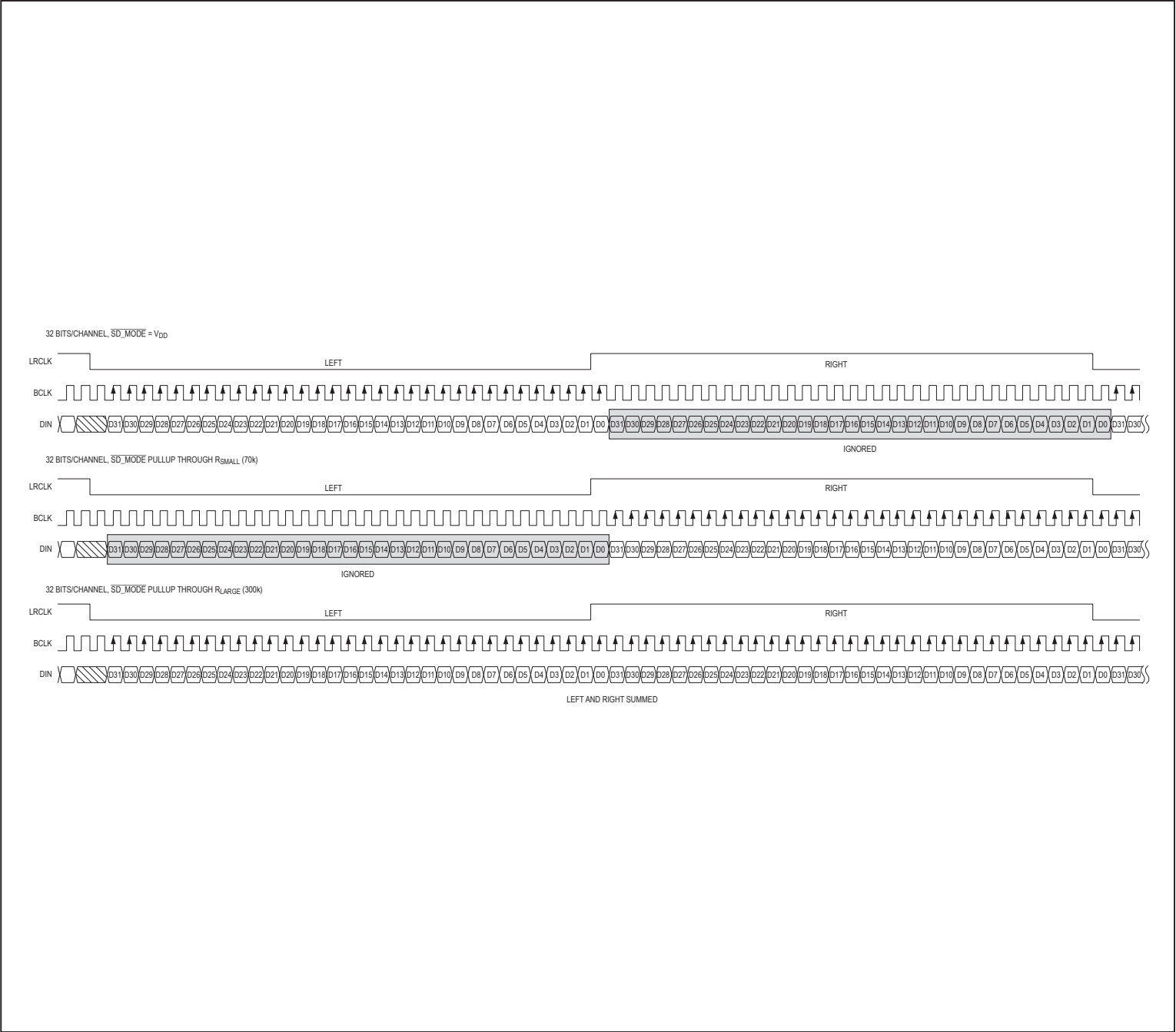
Figure 8. MAX98357A I2S Digital Audio Interface Timing, 32-Bit Resolution
