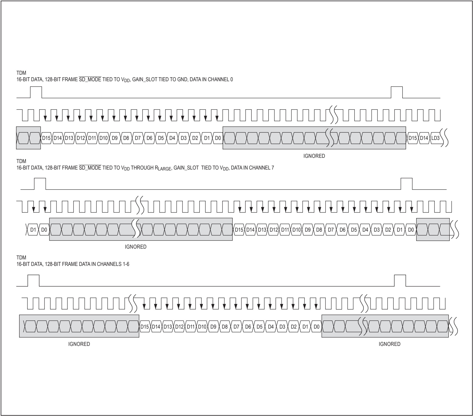
Figure 13. MAX98357B TDM 16-Bit DAI Timing
