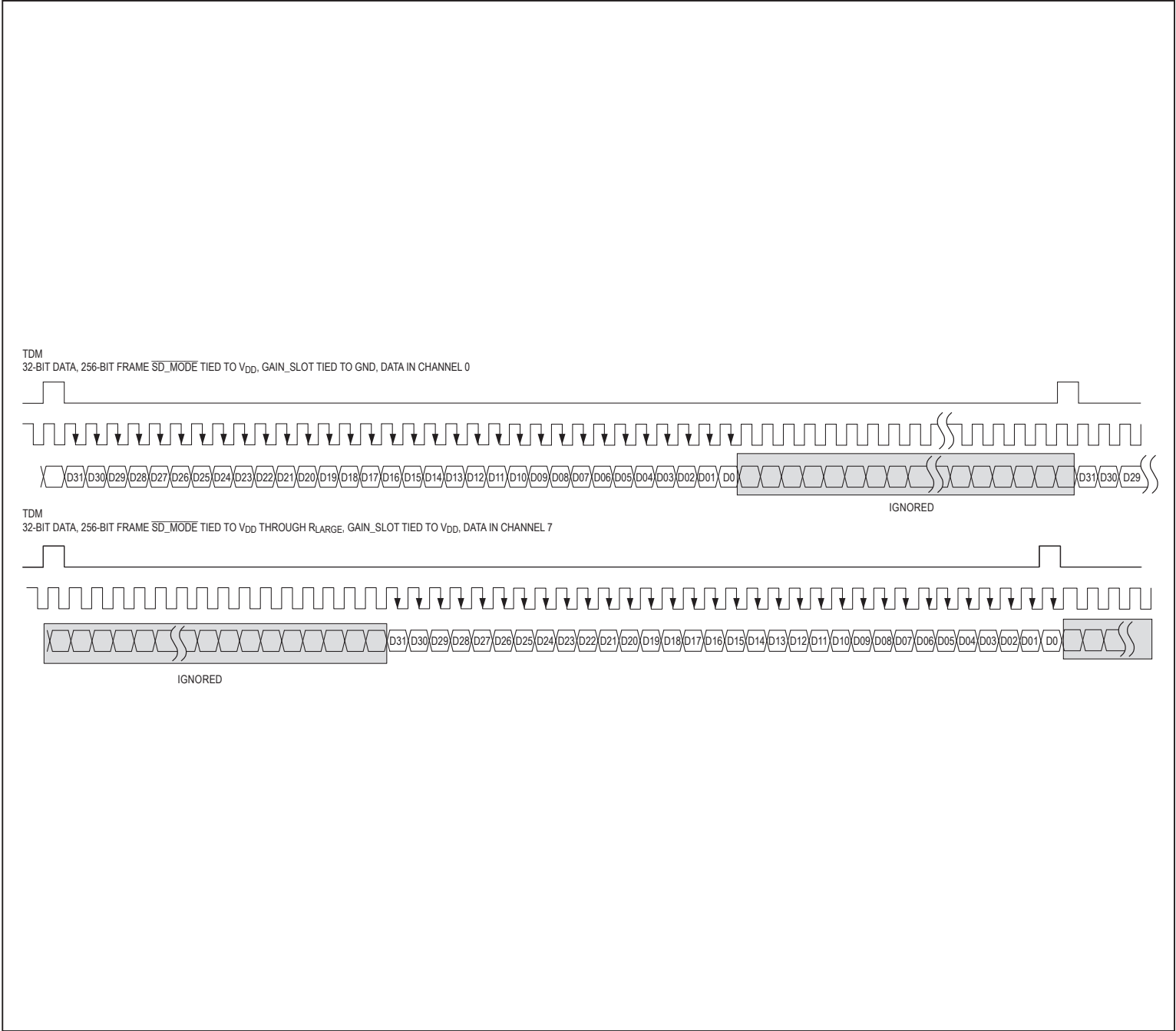
Figure 14. MAX98357B TDM 32-Bit DAI Timing
