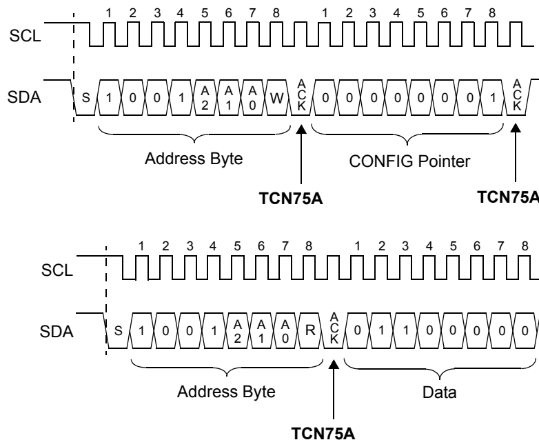
FIGURE 5-3: Timing Diagram for Writing and Reading from the Configuration Register (See Section 4.0 “Serial Communication” ).
