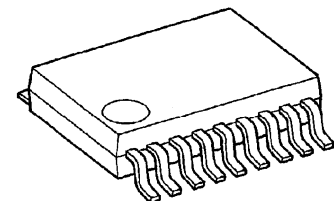
SSOP18-P-225-0.65
