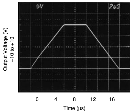
STEP RESPONSE
