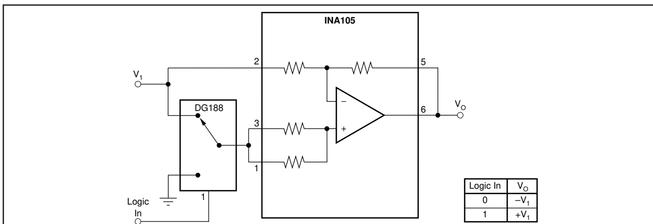
FIGURE 26. Digitally Controlled Gain of \pm 1 Amplifier.
