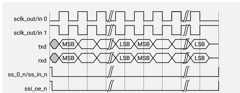
Figure 125. SPI Serial Format Continuous Transfer (SCPH = 1)
