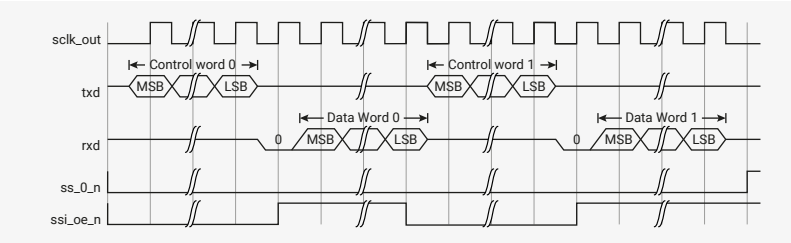
Figure 134. Continuous Nonsequential Microwire Transfer (receiving data frame)
