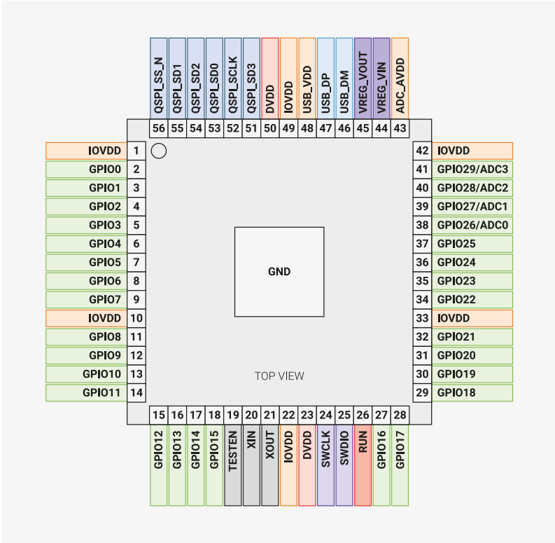
Figure 166. RP2040 QFN-56 package pinout
