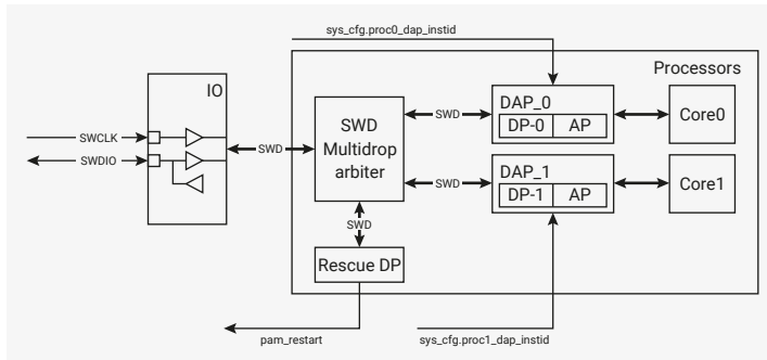
Figure 10. RP2040 Debugging
