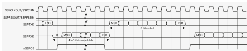
Figure 97. Microwire frame format, continuous transfers
