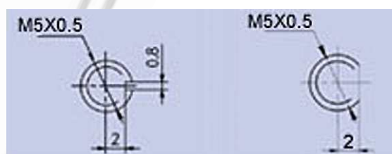
Standard ( ) Flat (F)
