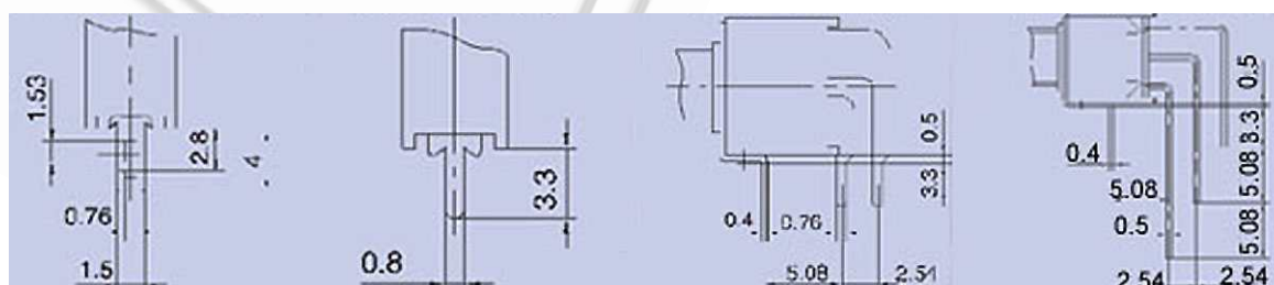
Solder terminal (1) PC terminal (2) PC-H terminal (3) PC-V terminal (4)
