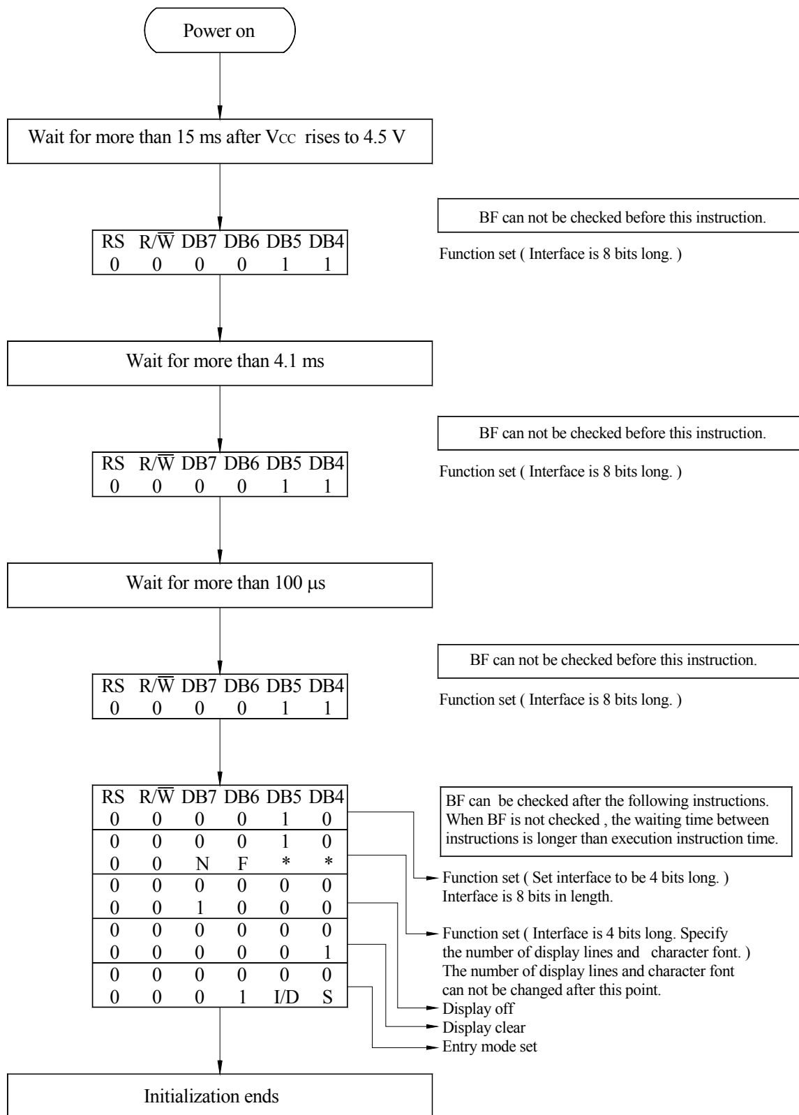
4-Bit Ineterface
