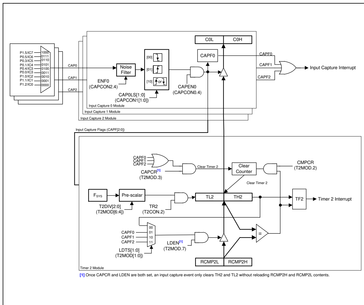
Figure 6.4-1 Timer 2 Block Diagram
