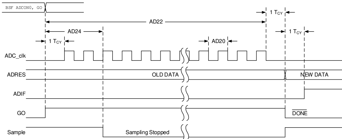
Figure 47-9. ADC Conversion Timing (ADC Clock F_{OSC} -Based)
