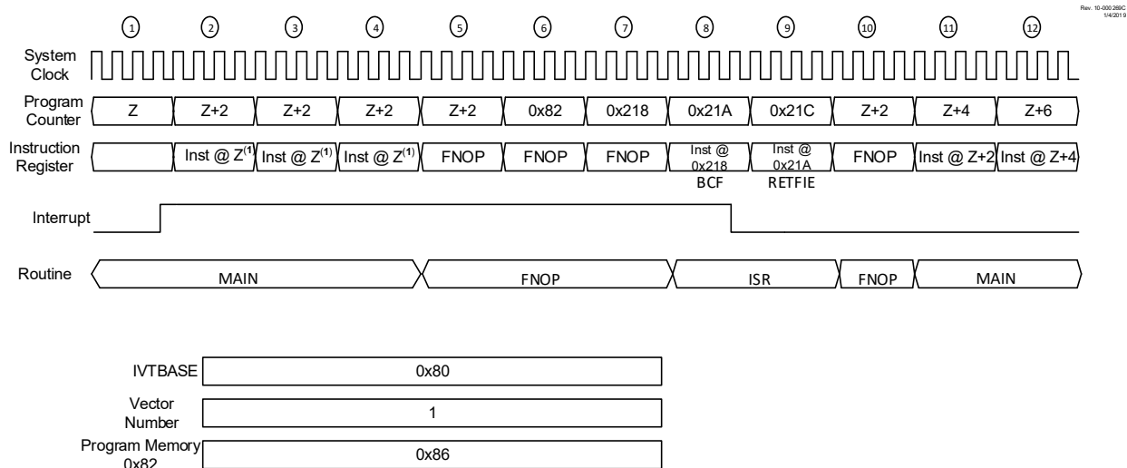
Figure 11-9. Interrupt Timing Diagram: Three-Cycle Instruction
