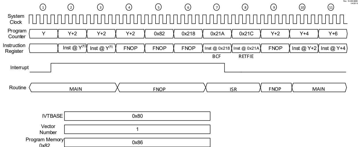
Figure 11-8. Interrupt Timing Diagram: Two-Cycle Instruction
