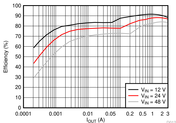
Efficiency Versus Output Current V_{OUT} = 5 V, f_{sw} = 500 kHz
