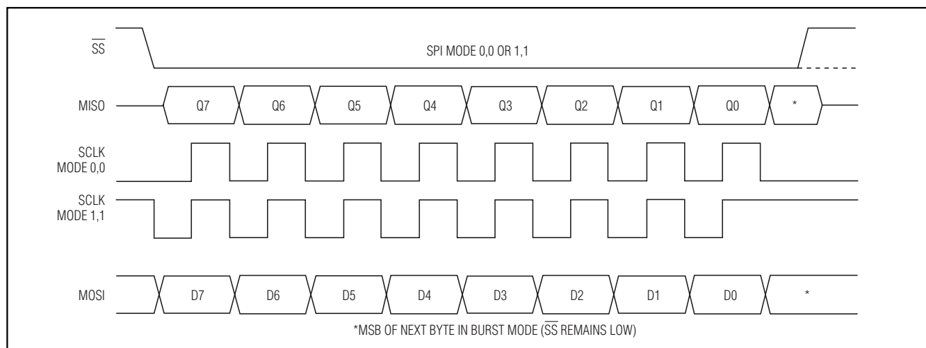
Figure 16. SPI Clocking Modes
