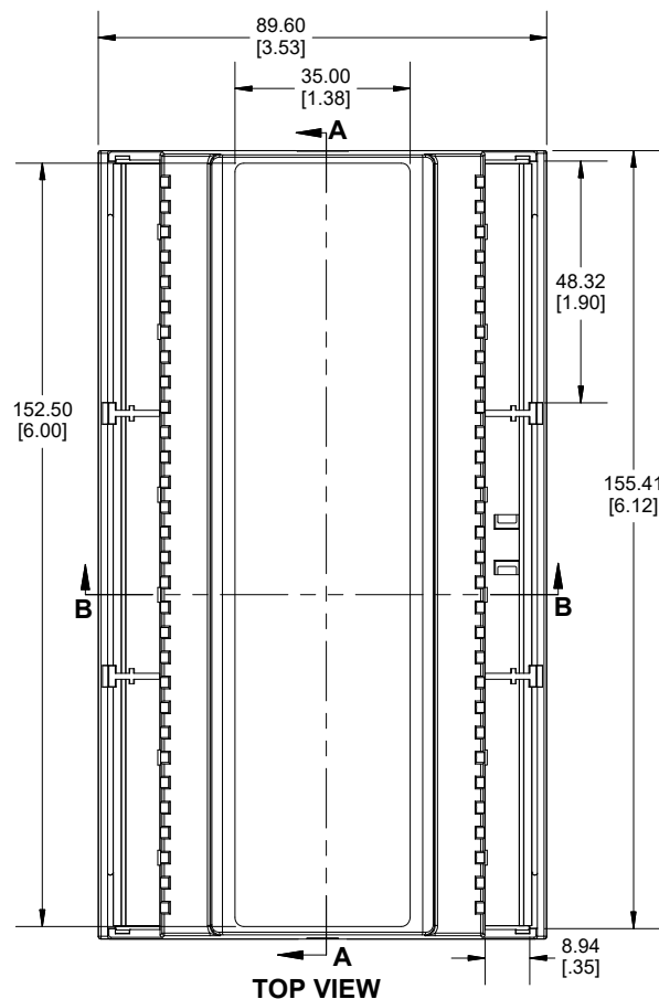
TOP VIEW
