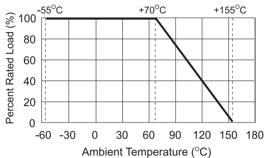
Derating Curve
