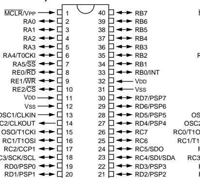
PIC16C64A PIC16CR64
