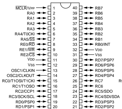
PIC16C64
