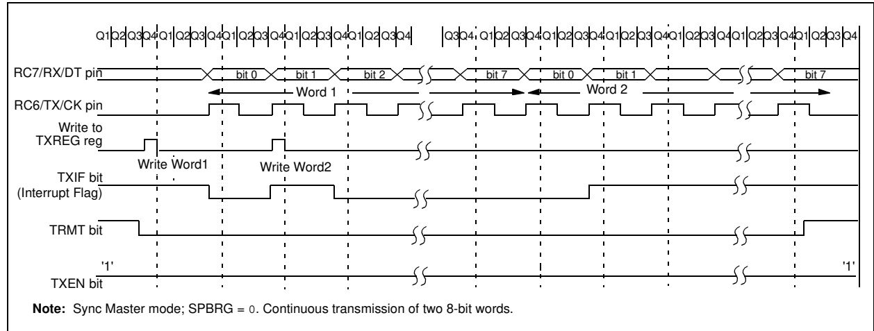
FIGURE 9-9: SYNCHRONOUS TRANSMISSION
