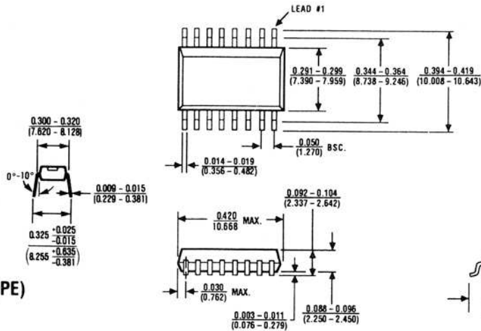
16 Lead Small Outline, Wide (WE)
