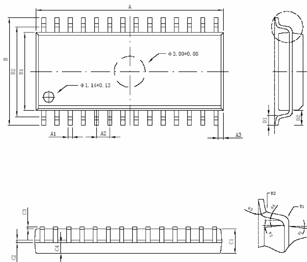
DETAIL "X"
