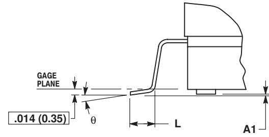
DETAIL G
