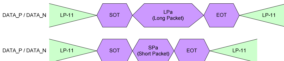
Figure 39: Single Packet in High-Speed Data Transmission
