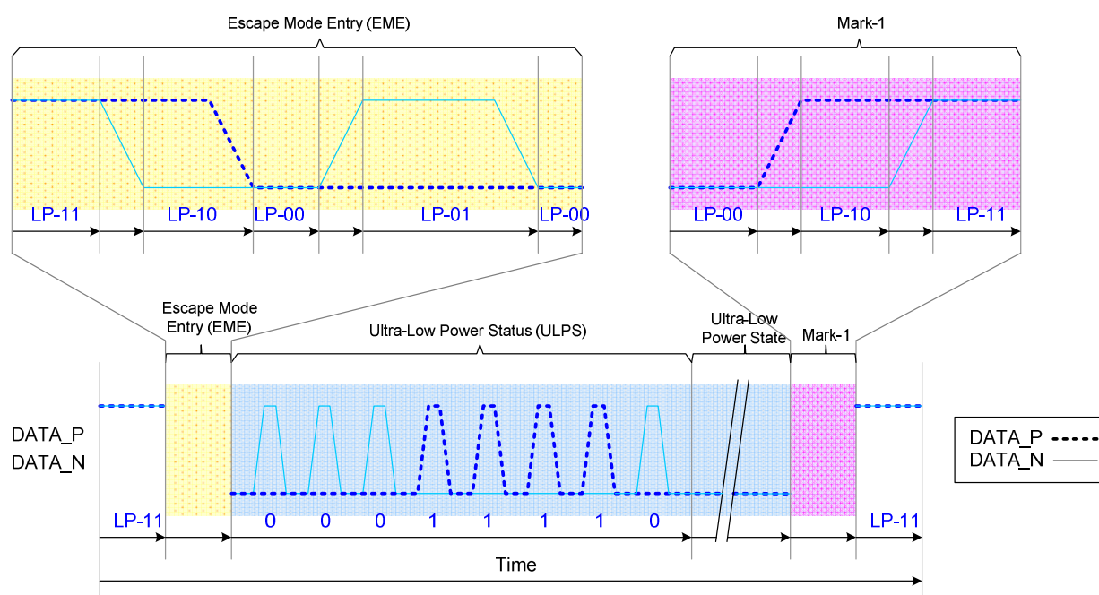
Figure 33: Ultra-Low Power State (ULPS)
