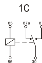
WIRING DIAGRAM (BOTTOM VIEW)
