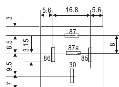
P.C.B LAYOUT (BOTTOM VIEW)
