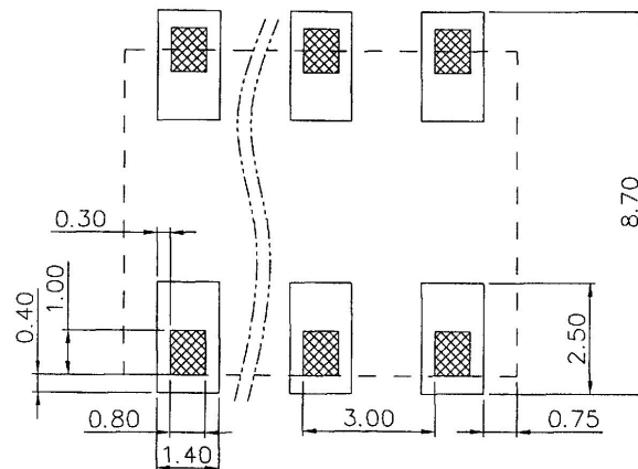
PCB LAYOUT
