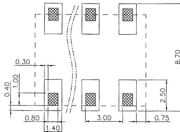
PCB LAYOUT
