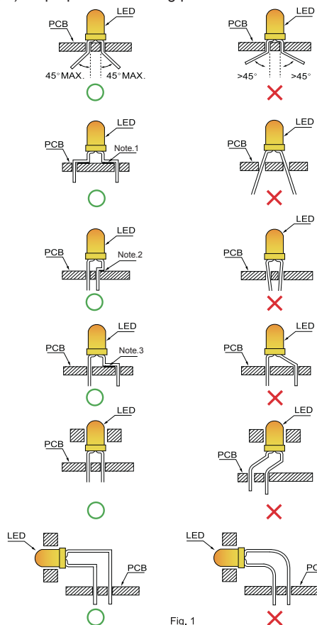
"O" Correct mounting method "X" Incorrect mounting method
