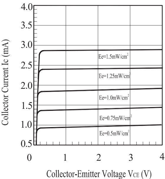
Fig.6 Collector Current vs. Collector-Emitter Voltage
