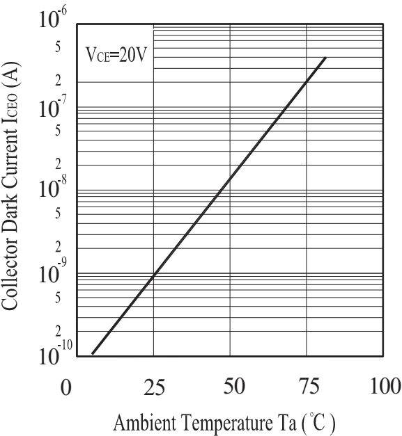
Fig.5 Collector Dark Current vs. Ambient Temperature
