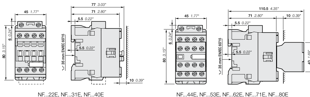
NF...22E, NF...31E, NF...40E
