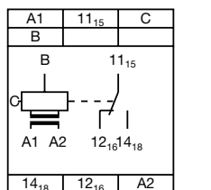
Connection diagram CM-ESS.1, CM-ESS.2
