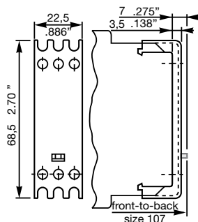
Sealable cover COV.01
