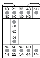
Combination 41E = NS/L31E/S + CA3-10/S
