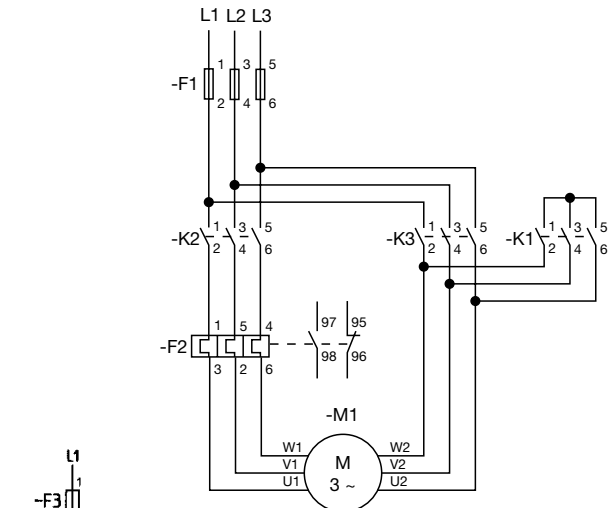
Power circuit diagram
