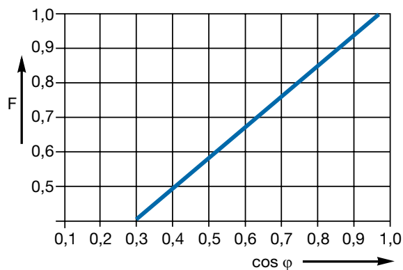
Derating factor F for inductive AC load
