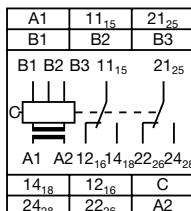
Connection diagram CM-SRS.M
