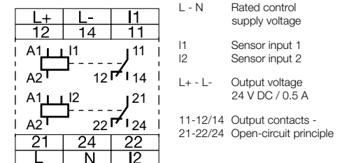
Connection diagram CM-SIS
