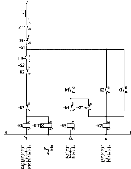
Control circuit diagram
