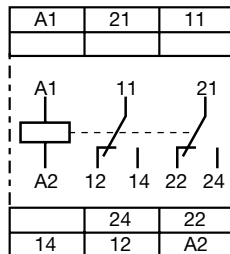
□ CT-IRS.24G (gold-plated cont.)
