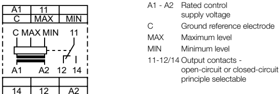
Connection diagram CM-ENS UP/DOWN
