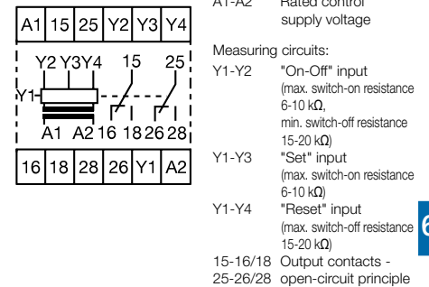
Connection diagram CM-KRN
