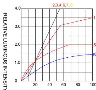
RELATIVE LUMINOUS INTENSITY VS FORWARD CURRENT
