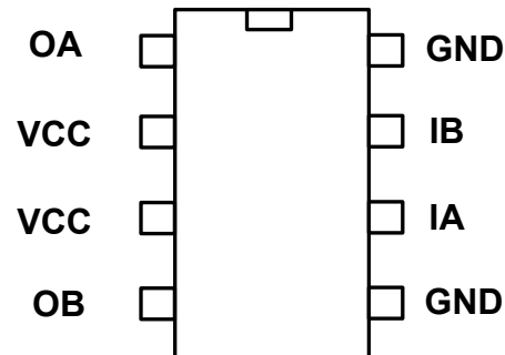
Device pins Figure
