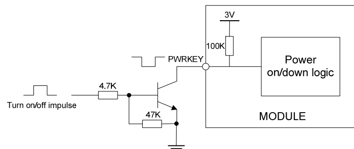
Figure 9: Powered on/down module using transistor
