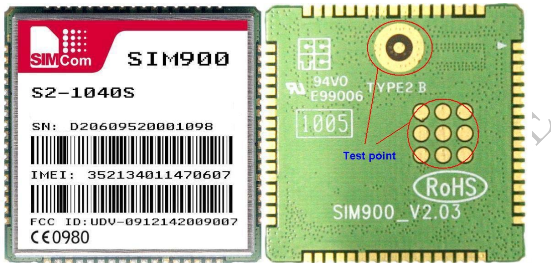
Figure 38: Top and bottom view of SIM900
