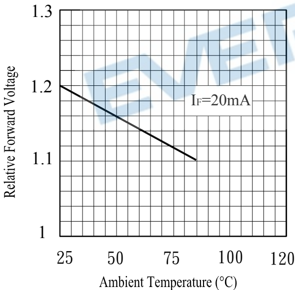
Relative Forward Voltage vs. Ambient Temperature
