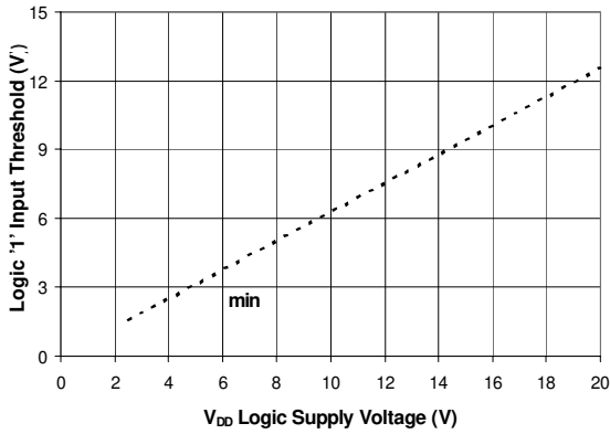
Figure 12B. Logic "1" Input Threshold vs. V_{DD} Voltage
