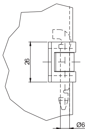
Mounting hole
