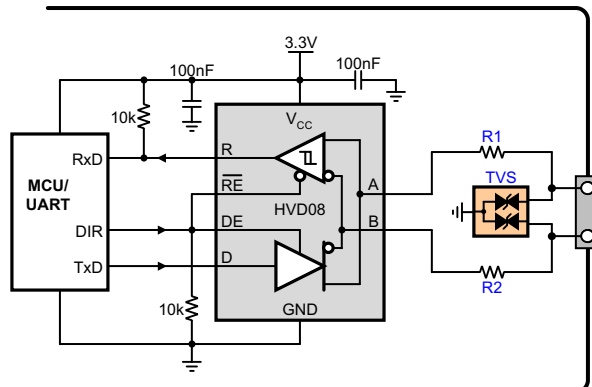
Figure 23. Transient protection against ESD, EFT, and Surge transients
