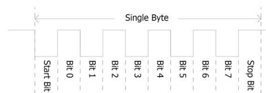
Figure 3.1: Single Byte Timing Diagram
