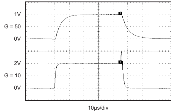
Figure 8. Step Response
