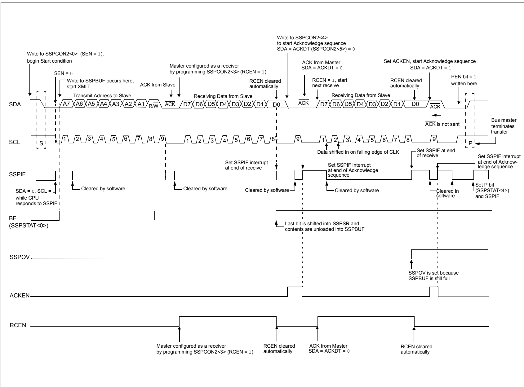
FIGURE 28-29: I 2 C MASTER MODE WAVEFORM (RECEPTION, 7-BIT ADDRESS)
