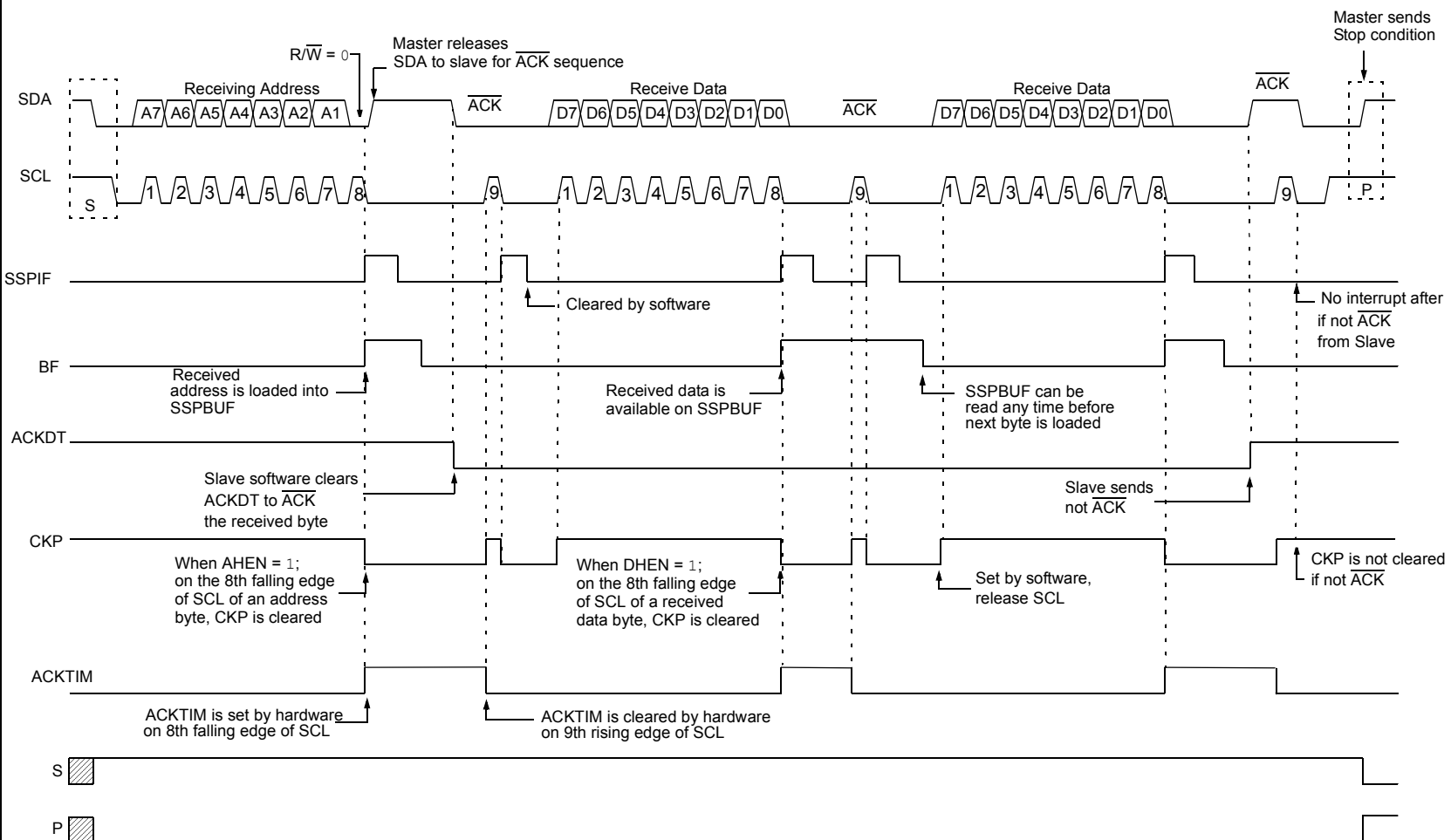
FIGURE 28-17: I 2 C SLAVE, 7-BIT ADDRESS, RECEPTION (SEN = 1, AHEN = 1, DHEN = 1)
