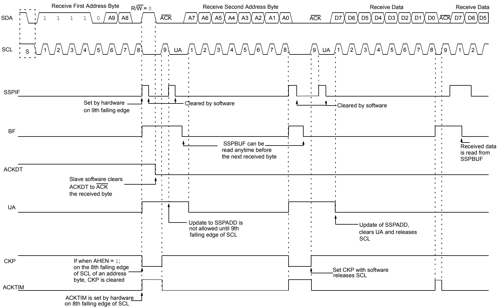
FIGURE 28-21: I 2 C SLAVE, 10-BIT ADDRESS, RECEPTION (SEN = 0, AHEN = 1, DHEN = 0)
