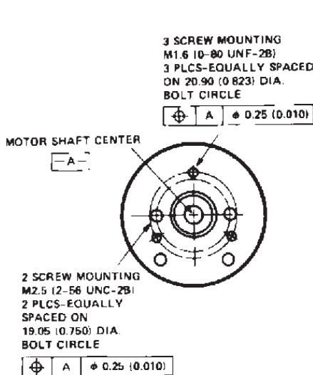
Figure 2. Mounting Holes.
