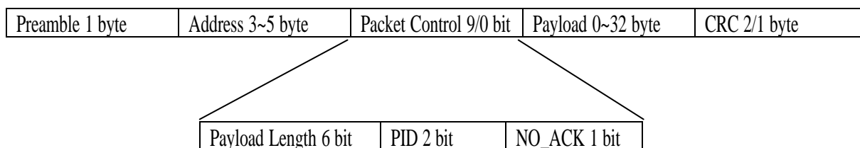
Figure 5 Packet Format
