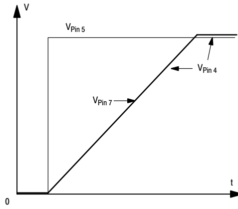
Figure 2. Acceleration Ramp
