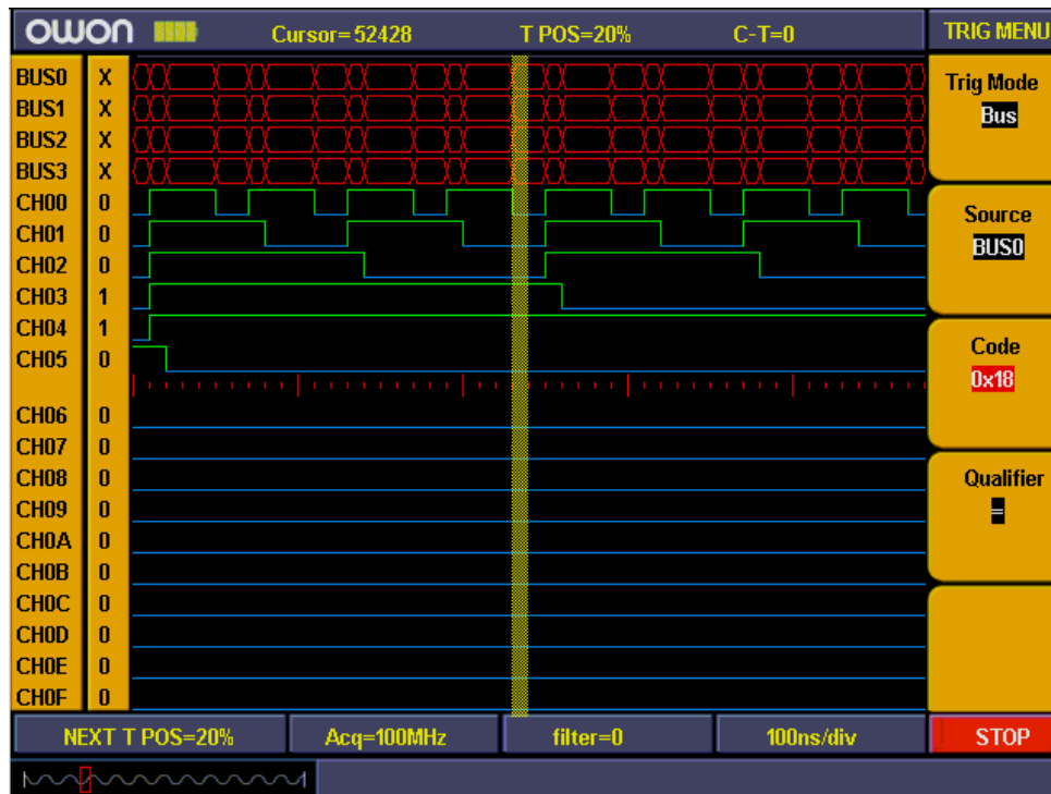
Fig 65: Bus trigger
