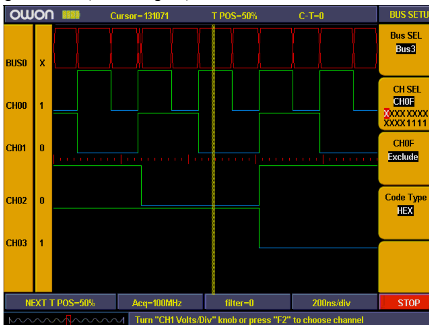
Fig 79: Bus setting
