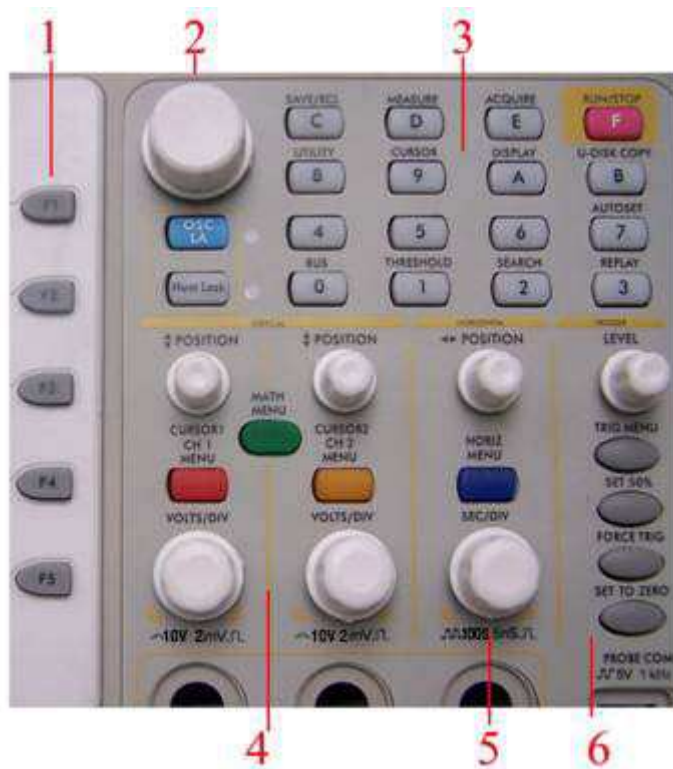
Fig 2: Keys Overview
