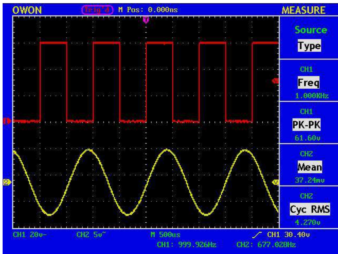
Fig. 56 Automatic Measurement
